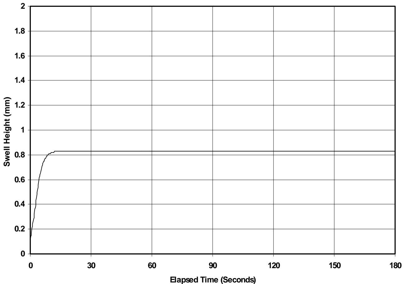
Swell Curve for 1069WB in DI Water
